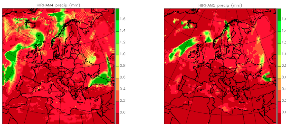
Figure 8. Precipitation for Europe, in mm. The figures show forecasts from equivalent HIRHAM4 (left) and HIRHAM5 (right) simulations.
