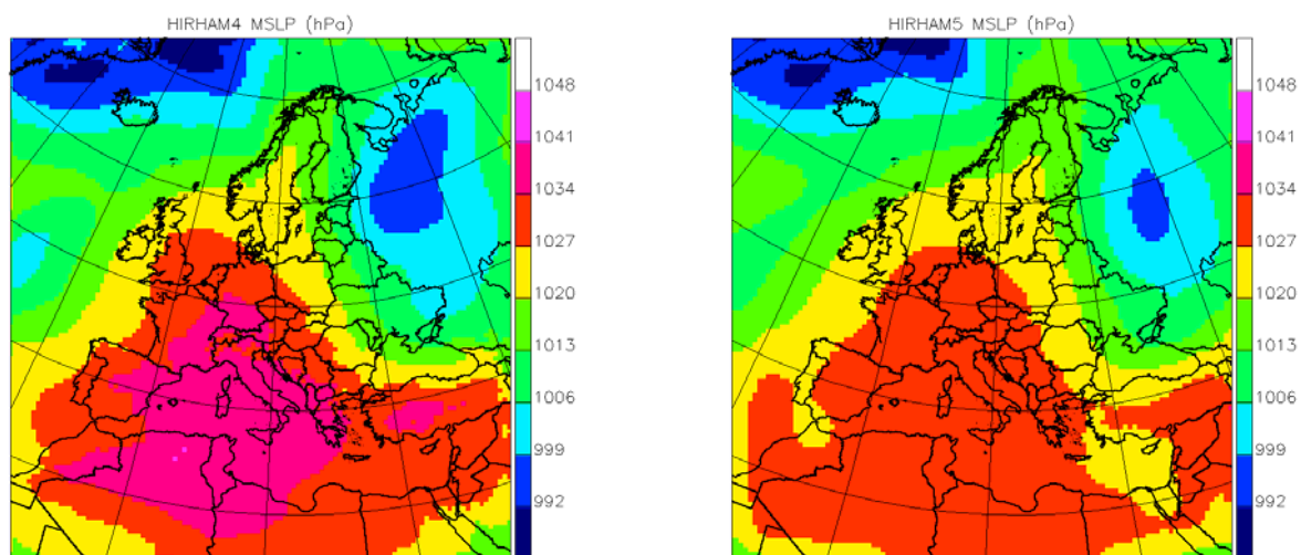
Figure 7. Mean sea level pressure (MSLP) for Europe, in hPa. The figures show results from equivalent HIRHAM4 (left) and HIRHAM5 (right) simulations.
