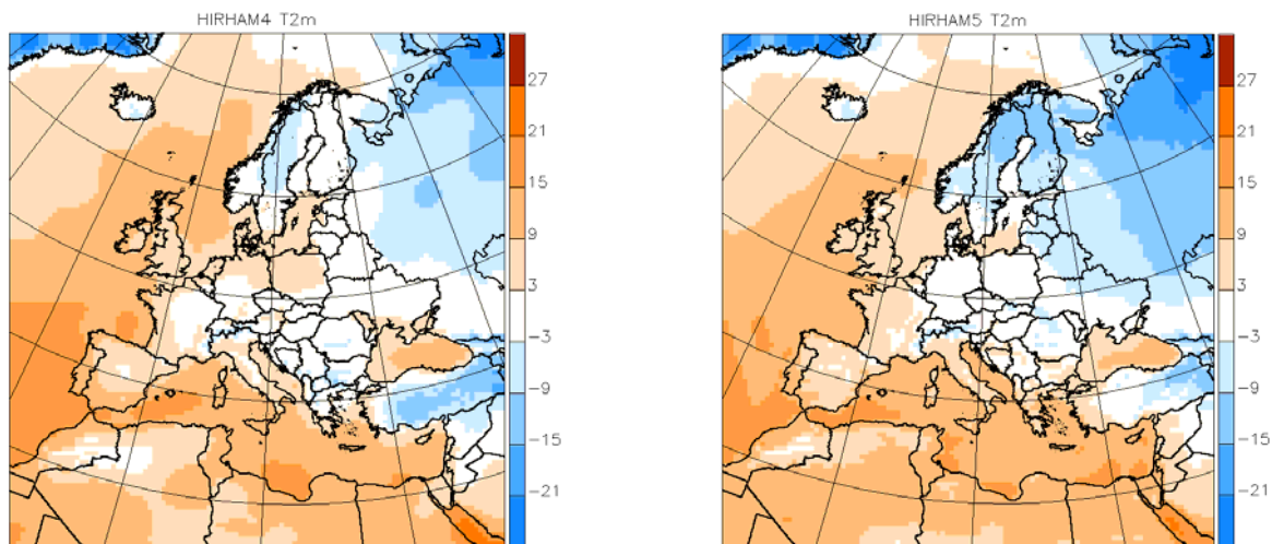
Figure 6. The 2-meter temperature (T2m) for Europe, in degrees Celsius for a January situation. The left column shows the result of a HIRHAM4 simulation, the right column the equivalent result for HIRHAM5.
